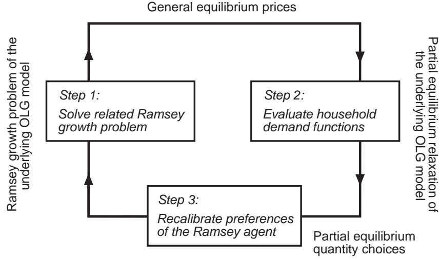
FIGURE 7: SOLVING OLG BY RAMSEY: STEPS IN THE DECOMPOSITION ALGORITHM
